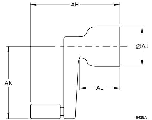
Detail of MA992A Tuning Handle
