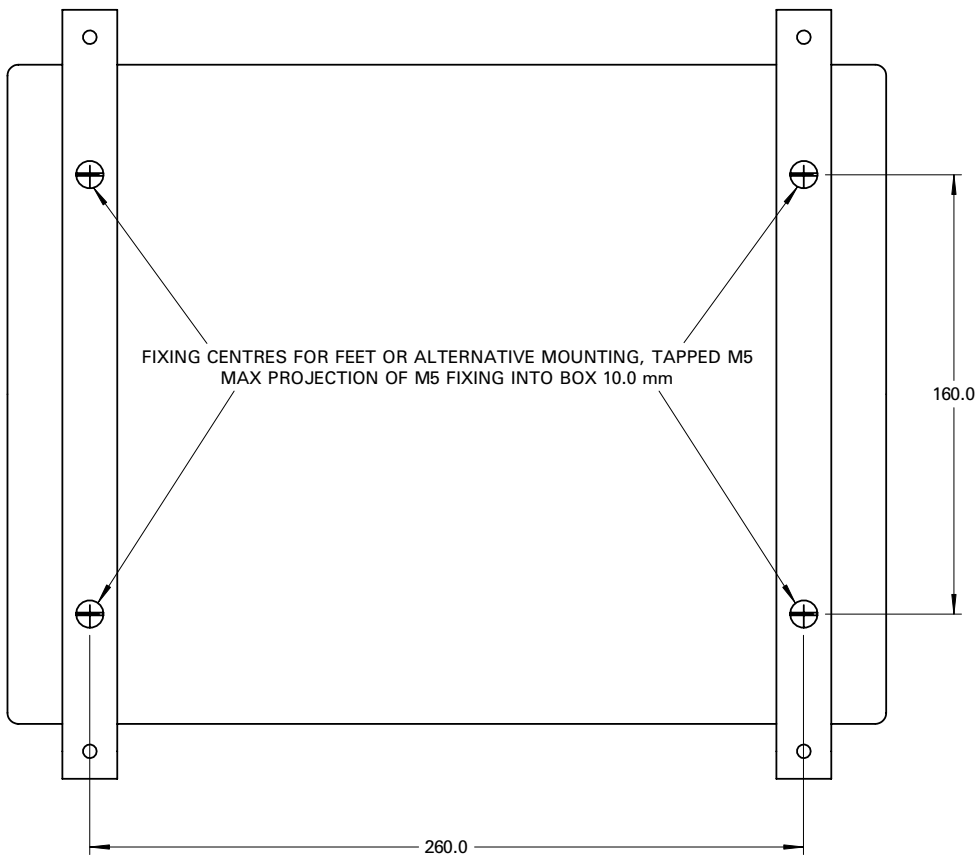
Fig. 3. Box layout and mounting (All dimensions nominal and in millimetres)
