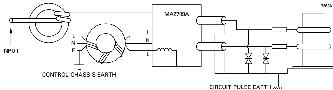
Fig. 2. MA2709A mounted close to the thyatron discharge circuit
